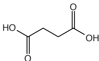
Succinic acid
